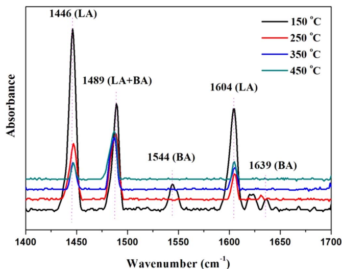
Fig. 1. Py-IR spectra of TS-1.
