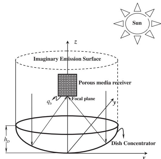
Fig. 1. Schematic diagram of the porous media receiver with solar dish collector system.
