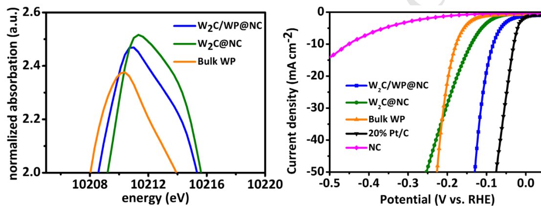
The XANES and polarization curves of HER for the different catalysts.
