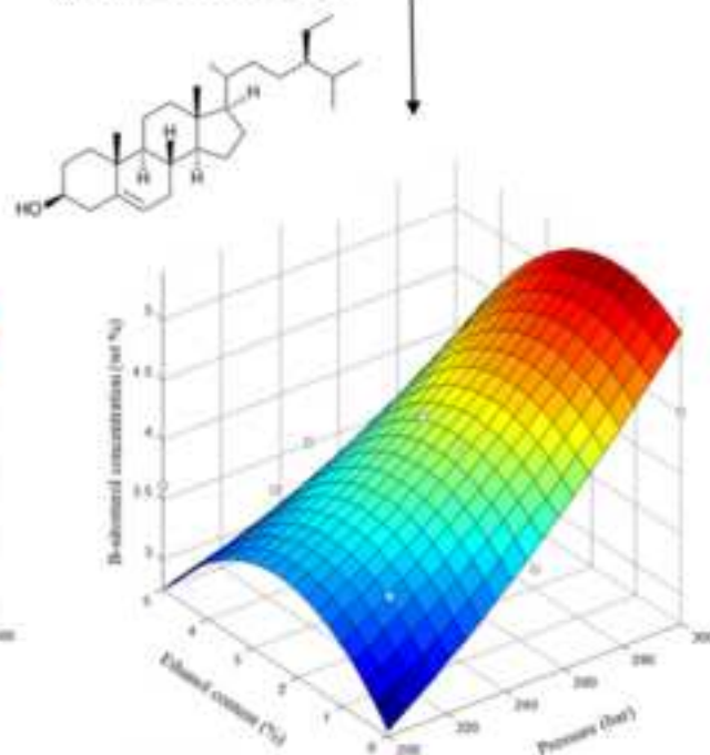
(c) \beta -Sitosterol
