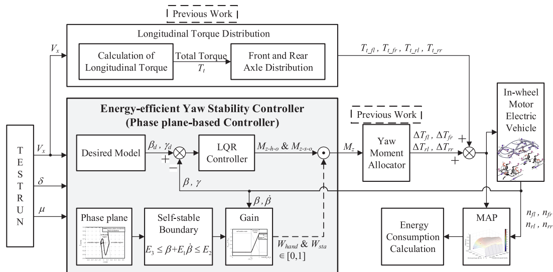
Fig. 1. Energy-efficient control system of electric vehicles.
