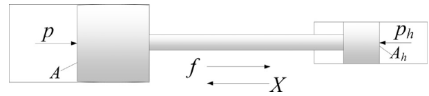
Fig. 1. Piston assembly force analysis.
