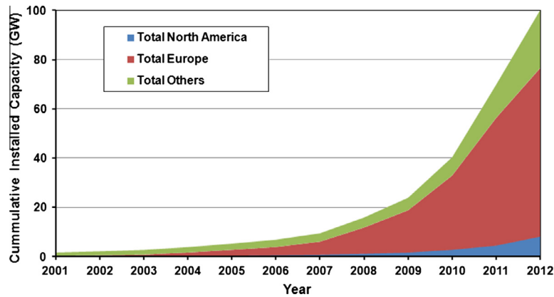
Fig. 1. Cumulative installed capacity of solar PV worldwide in 2011. Adapted from [1].
