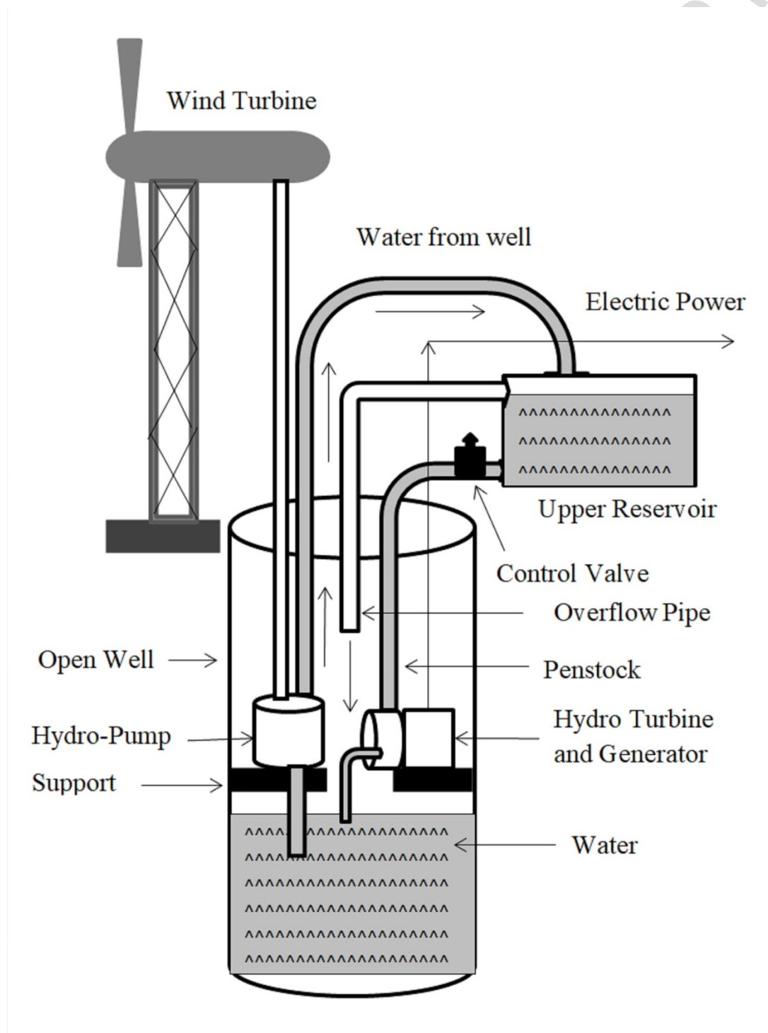
Fig. The proposed wind-PHES system
