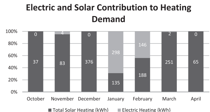
Fig. 1. Space heating demand for heating season analysed showing solar fraction.
