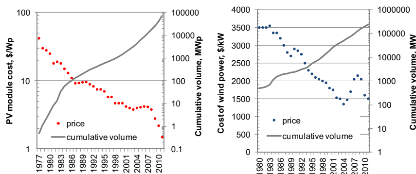
Fig. 1. Historical progress of PV and wind power. Costs and cumulative volumes shown.
