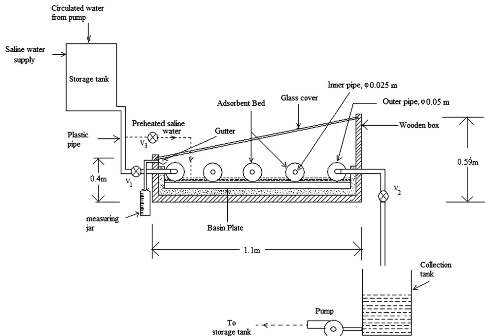
Fig. 1. Schematic diagram of the vapor adsorption type solar still.
