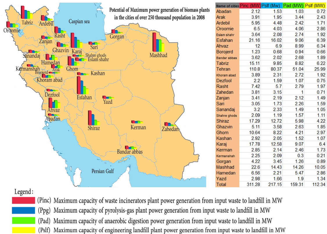
Fig. 1. Maximum potential of electricity generation in the various types of biomass-fuelled power plants in cities with populations of over 250000 (Renewable Energy and Energy Efficiency Organization of Iran).
