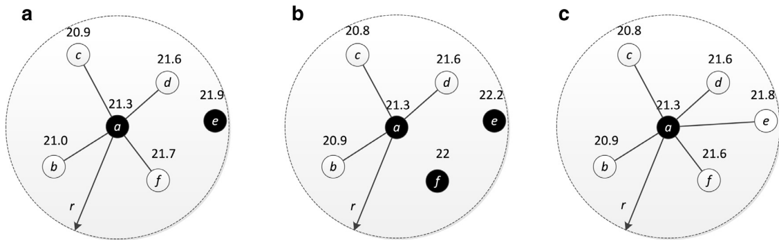
Fig. 1. An example for the representative nodes selection scheme: (a) using X , (b) using Y , (c) using Y' .
