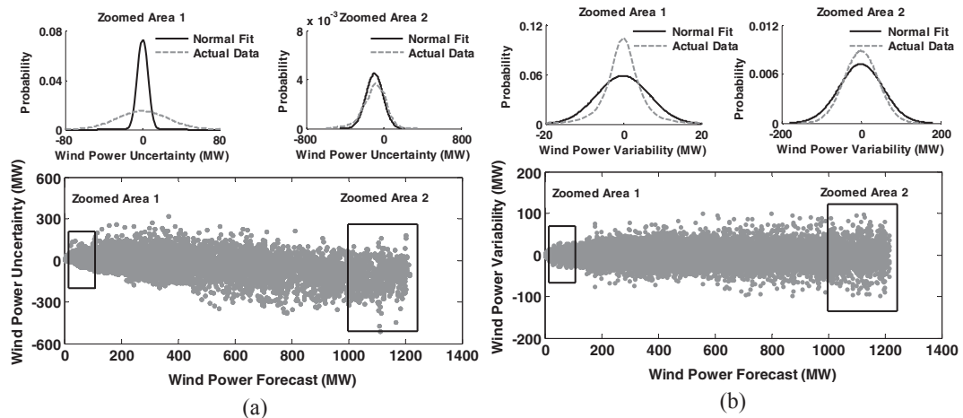
Fig. 1. (a) Wind power uncertainty (b) wind power variability as a function of wind power forecast in island of Ireland for year 2009.
