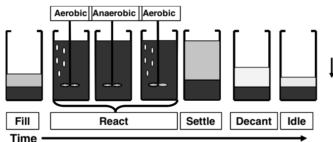
Fig. 1. SBR setup.
