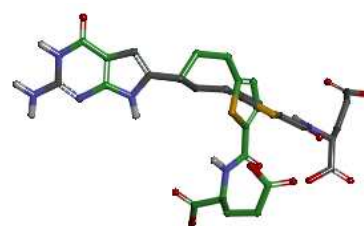
Superimposition of 1 (grey) in PCFT/Activity model (pharmacophore) over 10 (green) in RFC/Activity model (pharmacophore)
