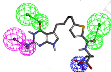
10 in RFC/Activity model (pharmacophore)
