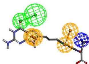
1 in PCFT/Activity model (pharmacophore)
