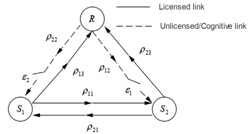
Fig. 2. Hybrid Cognitive Gaussian Two-Way Relay Channel (HCGTWRC) model.
