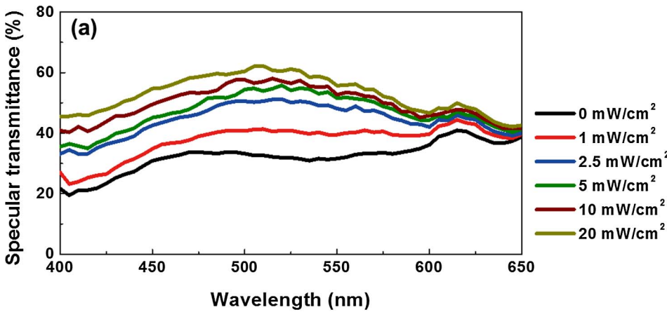
Fig. 1. Dependence of (a) specular transmission spectra and (b) images of dye-doped PS-ChLC cells on the UV intensity. Cell parameters; liquid crystals: E7, chiral dopant: S-811 (pitch: 1.25 μm), UV-curable monomer: RM 257 (2 wt%), photo-initiator: Irgacure 651 (0.1 wt%), black dichroic dye: S-428 (1 wt%), cell gap: 10 μm. The cell in the planar state was exposed to UV light for 10 min as we varied the intensity (0, 1, 2.5, 5, 10, and 20 mW/cm 2 ).
