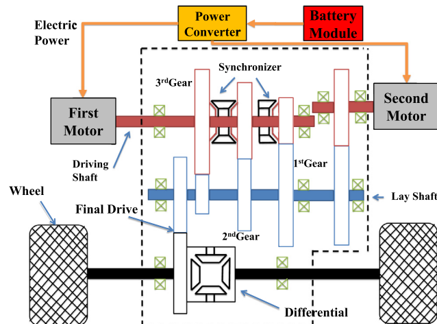
Fig. 1. Proposed dual input clutchless transmission system.
