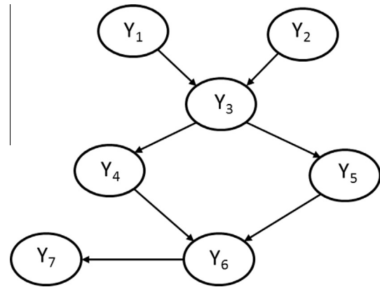
Fig. 2. A typical Bayesian network.
