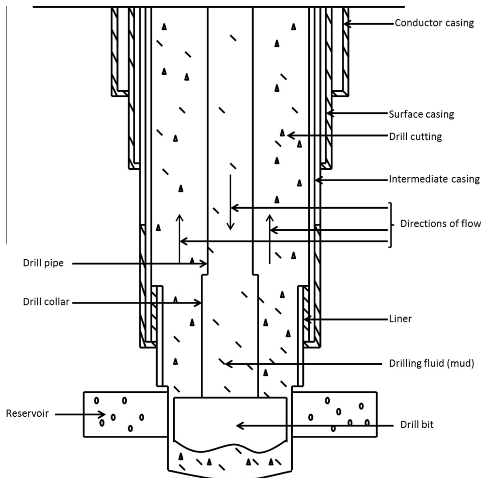
Fig. 1. A typical well profile.
