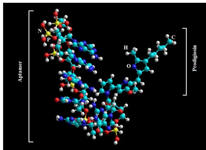
Fig. 2. Schematic diagram of conjugated aptamer.
