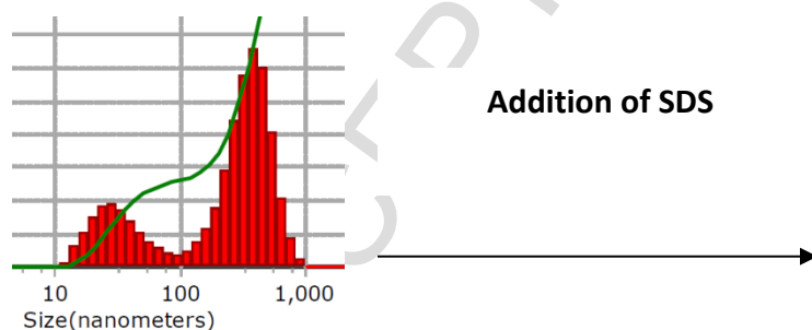
Molecular Size Distribution of Whey Protein Polymers
