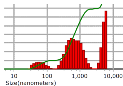
Molecular Size Distribution of SDS-Whey Protein Polymers Complex
