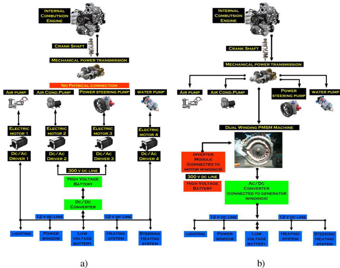
Fig. 1. (a) Drive by wire system, (b) proposed electrical accessory drive system.
