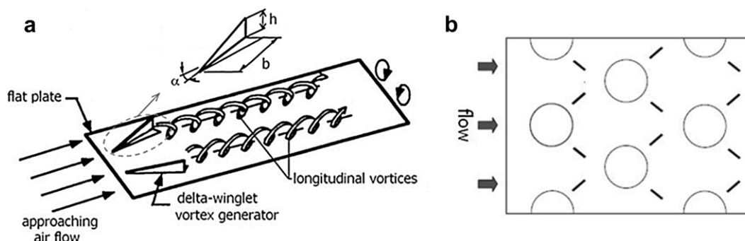
Fig. 2. (a) Delta winglet pair on a flat plate generating longitudinal vortices [7]; (b) Common-flow-down orientation of delta winglets on the fin of a round-tube heat exchanger [34].
