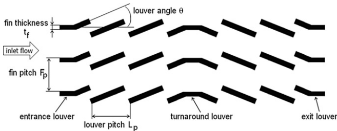
Fig. 1. Louvered fin design with main geometrical parameters.
