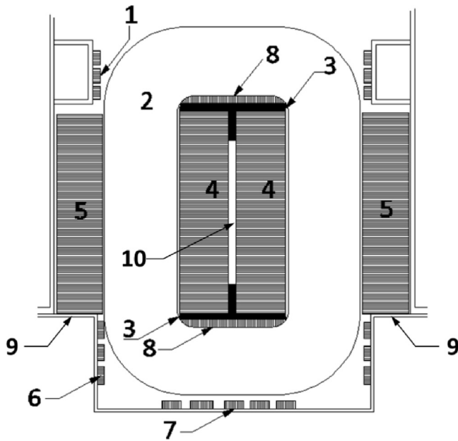
Fig. 1. Shell-form power transformer. 1: Side frame magnetic shunts, 2: pancake coils, 3: T-beams, 4: tongue iron, 5: leg iron, 6: end tank magnetic shunts, 7: tank bottom shunts, 8: T-beams magnetic shunts, 9: supports of the end tank, 10: supports between T-beams.
