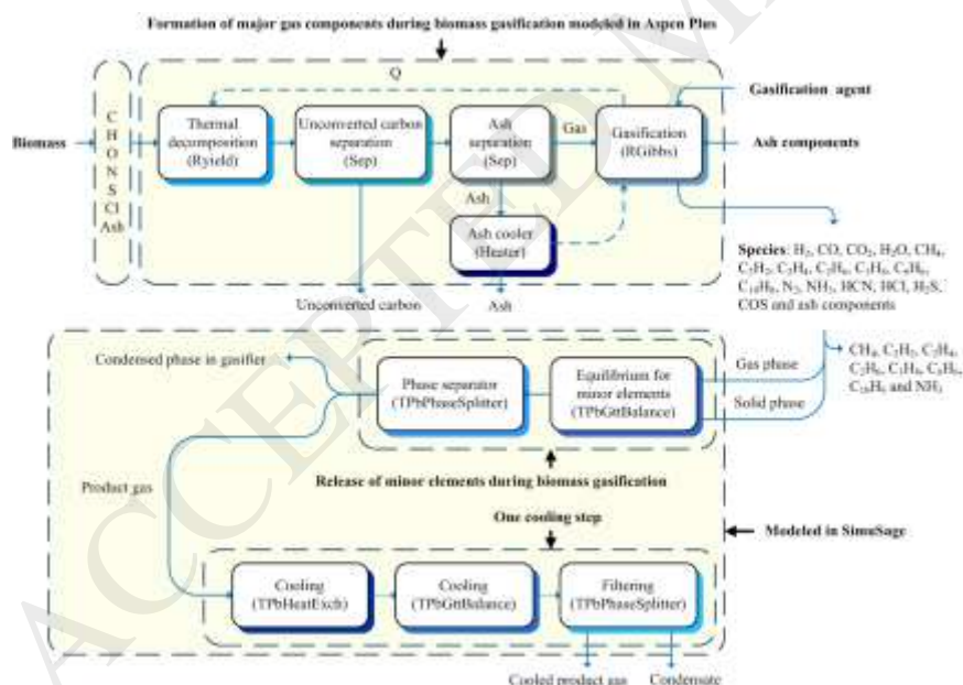
Fig. 1 Schematic diagram of the model developed by combining Aspen Plus with SimuSage
