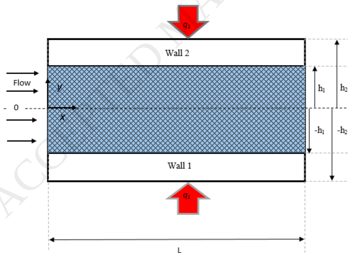
Fig. A. Schematic view of the investigated microreactor.
