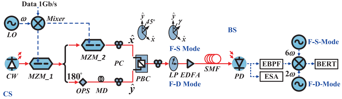
Fig. 1. Schematic diagram of the proposed optical MMW generator based RoF system. CS, center station (CW, continuous wave laser; LO, local oscillator; MZM, Mach-Zehnder modulator; OPS, optical phase shifter; MD, Matching delay; PC, polarization controller; PBC, polarization beam combiner; LP, linear polarizer; EDFA, Erbium-doped fiber amplifier); SMF, Single mode optical fiber; BS: base station (PD, photodiode; ESA, electrical spectrum analyzer; EBPF, electrical band-pass filter; BERT, bit error rate tester); F-D mode, frequency-doubling mode; F-S mode, frequency-sextupling mode.
