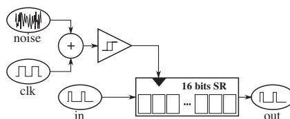
Fig. 1. Noise-tunable delay line.
