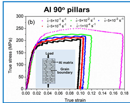
Transition in deformation mechanism with the increasing strain rates
