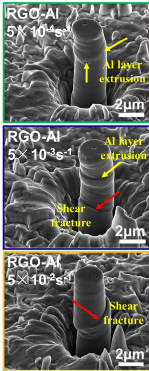
Transition in deformation mechanism with the increasing strain rates
