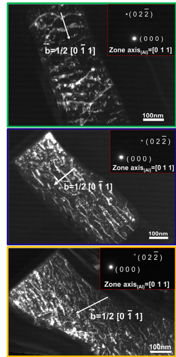
Transition in deformation mechanism with the increasing strain rates
