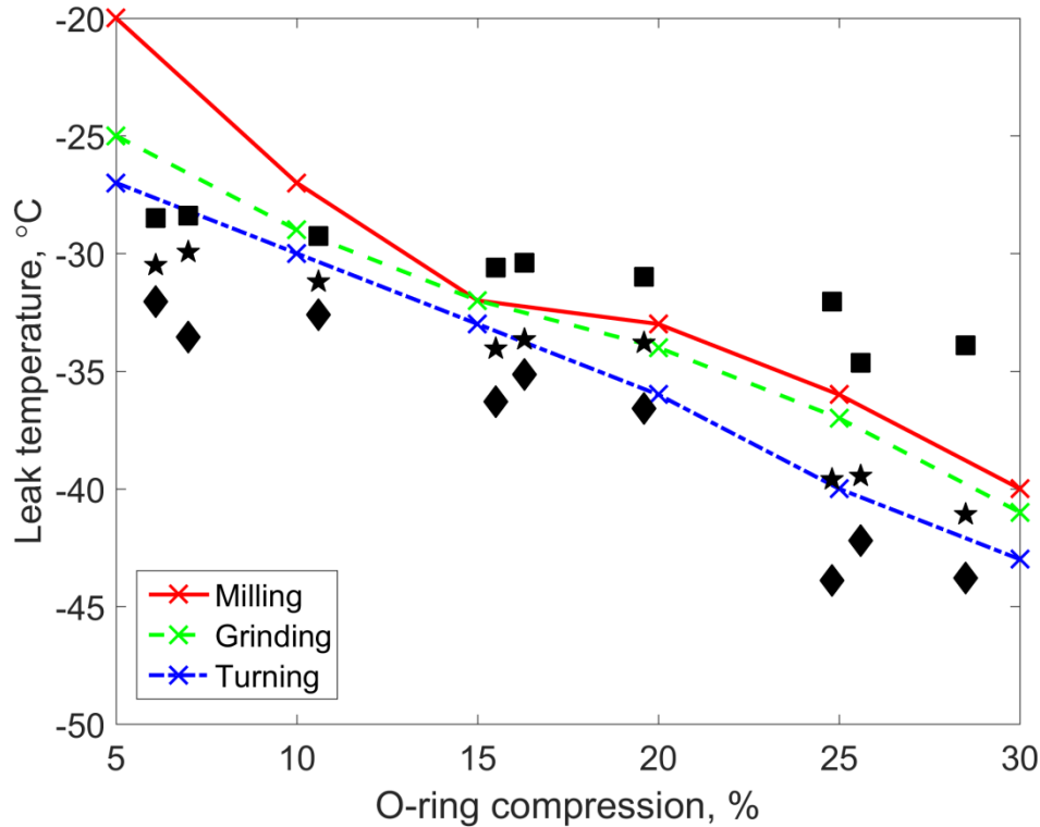
Prediction of cold seal failures vs experiment
