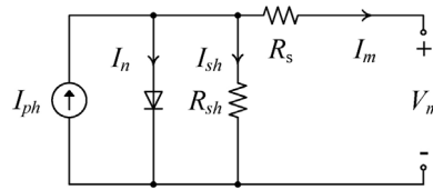
Fig. 1. Equivalent circuit of the single diode model.
