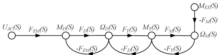
Fig. 1. Mason graph of studied EMS with SE.
