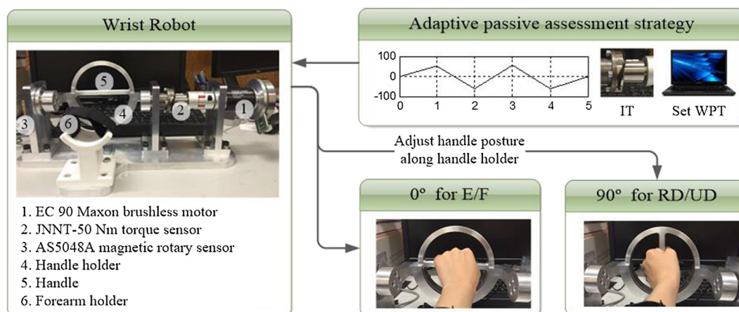
Fig. 1. A reconfigurable wrist rehabilitation robot. (IT: Interaction torque; WPT: Wrist passive torque; E/F: Extension/flexion; RD/UD: Radial/ulnar deviation).
