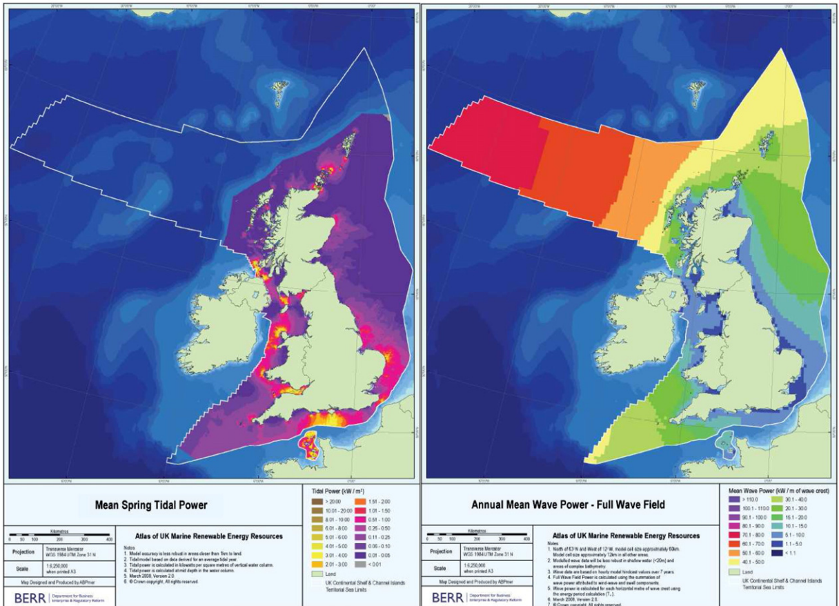
Fig. 1. Average tidal power and mean wave power in the UK (source: [12]).
