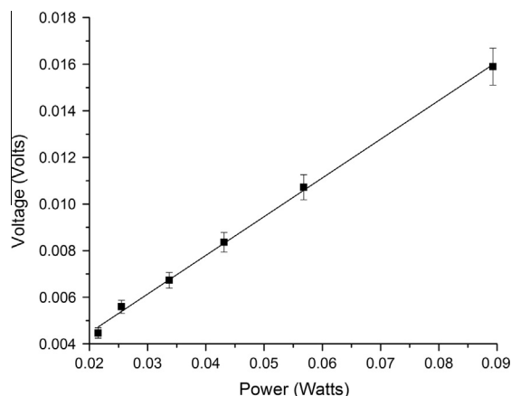
Fig. 2. Plot of measured voltage as a function of laser power. Best fit equation: y = 0.16612x + 0.00116 , R^2 = 0.99804 .
