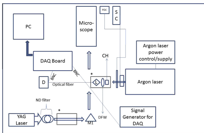
Fig. 1. The schematic of the experimental setup. M1 represents the horizontal turning mirror which directs the beam into the inverted microscope where it arrives at the sample and can be moved to line up with the Ar + -ion laser as needed. SC is the shutter control (Thorlabs SH05 and SC10, $1070), CH is the cuvette holder, DFW is the dichroic filter wheel, ND represents the neutral density filters, D is the detector (Thorlabs DET02AFC, $269) and L is the collimator (Cable: Thorlabs M65L01, $105; Collimator: Thorlabs F810SMA-543, $196).
