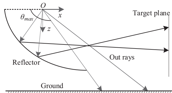
Fig. 4. Schematic diagram of the reflected lighting system.
