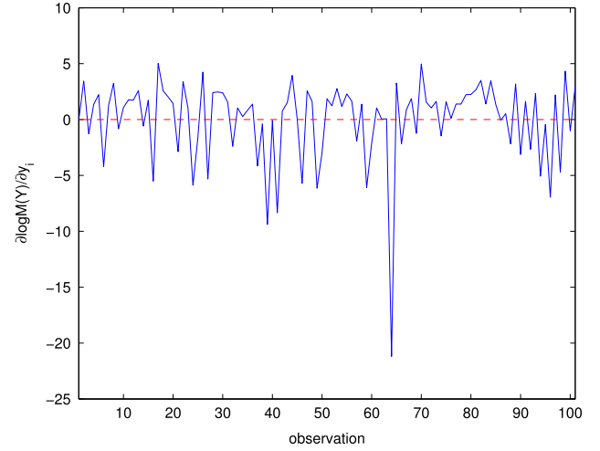
Fig. 1. Local sensitivity of log marginal likelihood.
