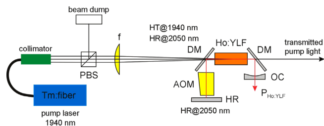
Fig. 1. Experimental setup of the end-pumped Ho:YLF laser: PBS – polarizing beam splitter, DM – flat dichroic mirrors anti-reflective at 1.94\ \mu\text{m} and 45\text{-deg} highly reflective at 2.05\ \mu\text{m} , OC – concave output-coupling mirror, AOM – acousto-optic modulator, HR – high reflector.
