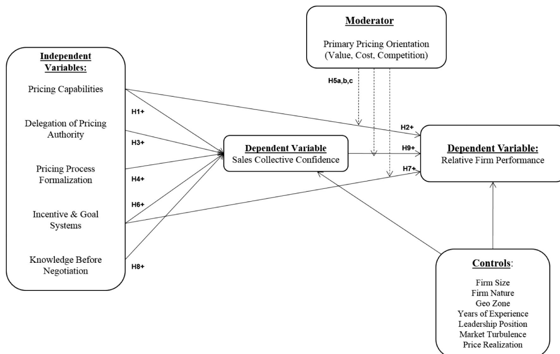
Fig. 1. Hypothesized research model.
