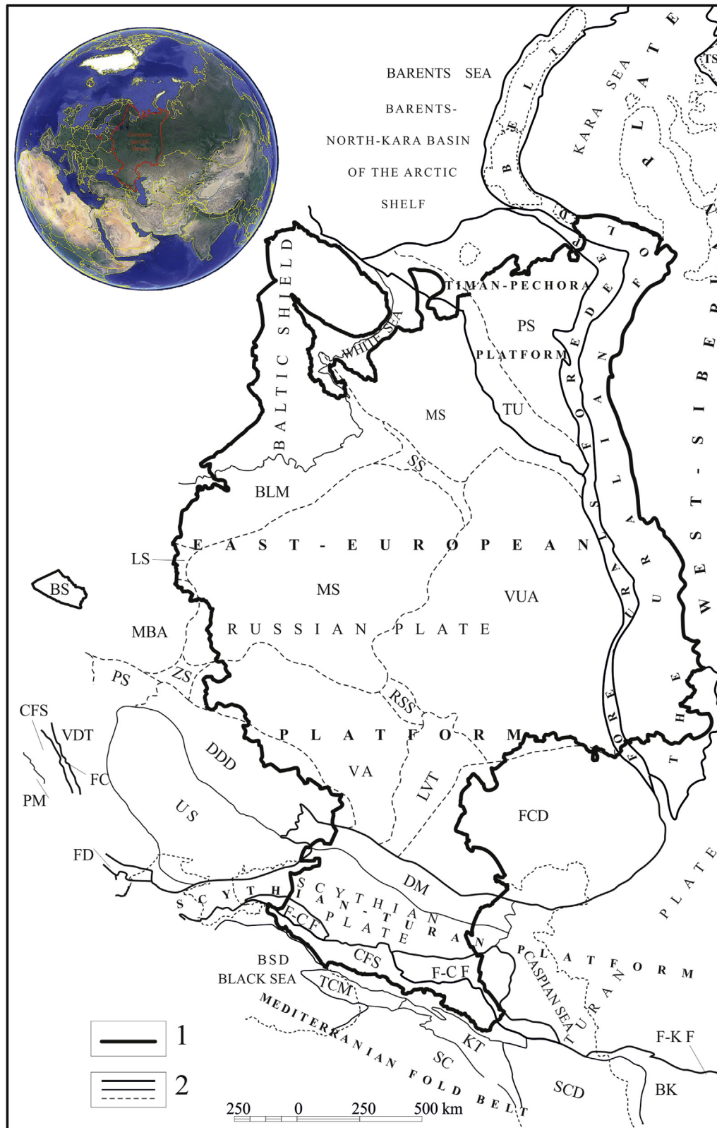
Fig. 1. General map (A) and Scheme of the tectonic zonation of the European part of Russia (B) (By Strelnikov in Geological map ... , 2012, modified by authors). Legend: 1. Boundary of the territory discussed in the paper; 2. Boundaries of the tectonic structures of different levels. Tectonic zonation. East-European Platform: BLM – Baltic – Ladoga Monocline; BS – Baltic Syncline; DDD – Dnieper – Donetsk Depression; FCD – Fore-Caspian Depression; LS – Latvian Saddle; LVT – Lower Volga Trough; MBA – Mazurian – Belarussian Antecline; MS – Mezen Syncline; MS – Moscow Syncline; PS – Polesk Saddle; RSS – Ryazan-Serdobsk Saddle; SS – Sukhona Saddle; US – Ukrainian Shield; VA – Voronezh Antecline; VDT – Visla – Dniester Trough; VUA – Volga – Urals Antecline; ZS – Zhlobin Saddle; 4. Mediterranean Fold Belt: BK – Balkan – Kopetdag Fold System; BSD – Black Sea Depression; CFS – Caucasus Fold System; KT – Kura Trough; SCD – South Caspian Depression; TCM – Trans-Caucasian Massif; SC – Small Caucasus Fold-block System; 5. Timan-Pechora Platform: PS – Pechora Syncline; TU – Timan Uplift; 6. Scythian-Turan Platform: DM – Donetsk-Mangyshlak Fold Area; 7. FC – Fore-Carpathian Trough; FD – Fore-Dobrudja Trough; TSZ – Taimyr-Severnaya Zemlya Fold System; 8. F-C F- Fore-Caucasian Foredeep; F-K F – Fore-Kopetdag Foredeep.
