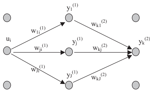
Fig. 1. Feedforward neural network outline.
