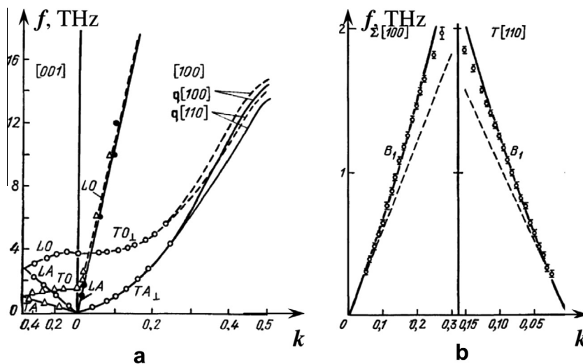
Fig. 2. Quadratic phonon dispersion in graphite (a) and linear phonon dispersion in GaS (b). The wavenumber is given in relative units.
