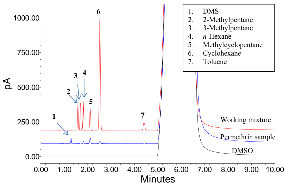
Representative Chromatograms of the Final Method (Column: DB-1, 15 m x 0.53 mm I.D., 3.0 \mu m film thickness)
