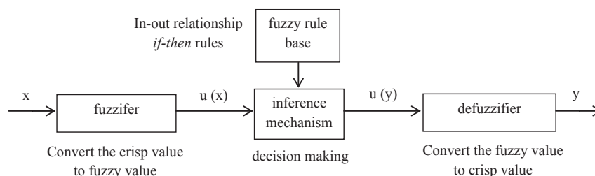
Fig. 1 – Schematic of fuzzy logic system.
