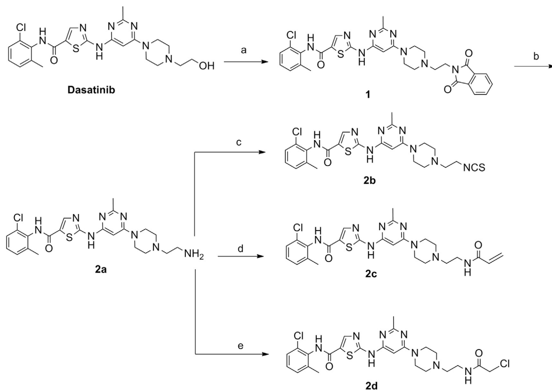
Scheme 1. Reagents and conditions: (a) \text{PPh}_3 , phthalimide, DIAD, THF, r.t., 88%; (b) \text{N}_2\text{H}_2\cdot\text{H}_2\text{O} , EtOH, 78 °C, 72%; (c) DCC, \text{CS}_2 , \text{CH}_2\text{Cl}_2 , r.t., 52%; (d) acryloyl chloride, \text{Et}_3\text{N} , \text{CH}_2\text{Cl}_2 , r.t., 49%; (e) chloroacetyl chloride, \text{Et}_3\text{N} , \text{CH}_2\text{Cl}_2 , r.t., 55%;
