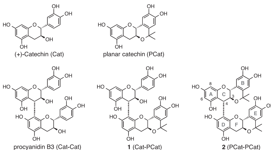
Fig. 1. Structures of (+)-catechin, planar catechin, procyanidin B3 (Cat-Cat), and procyanidin B3 derivatives 1 (Cat-PCat) and 2 (PCat-PCat).
