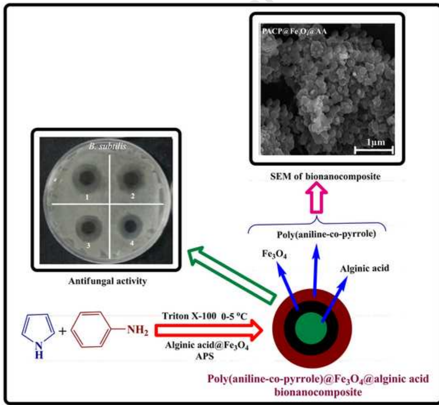
Graphical abstract
