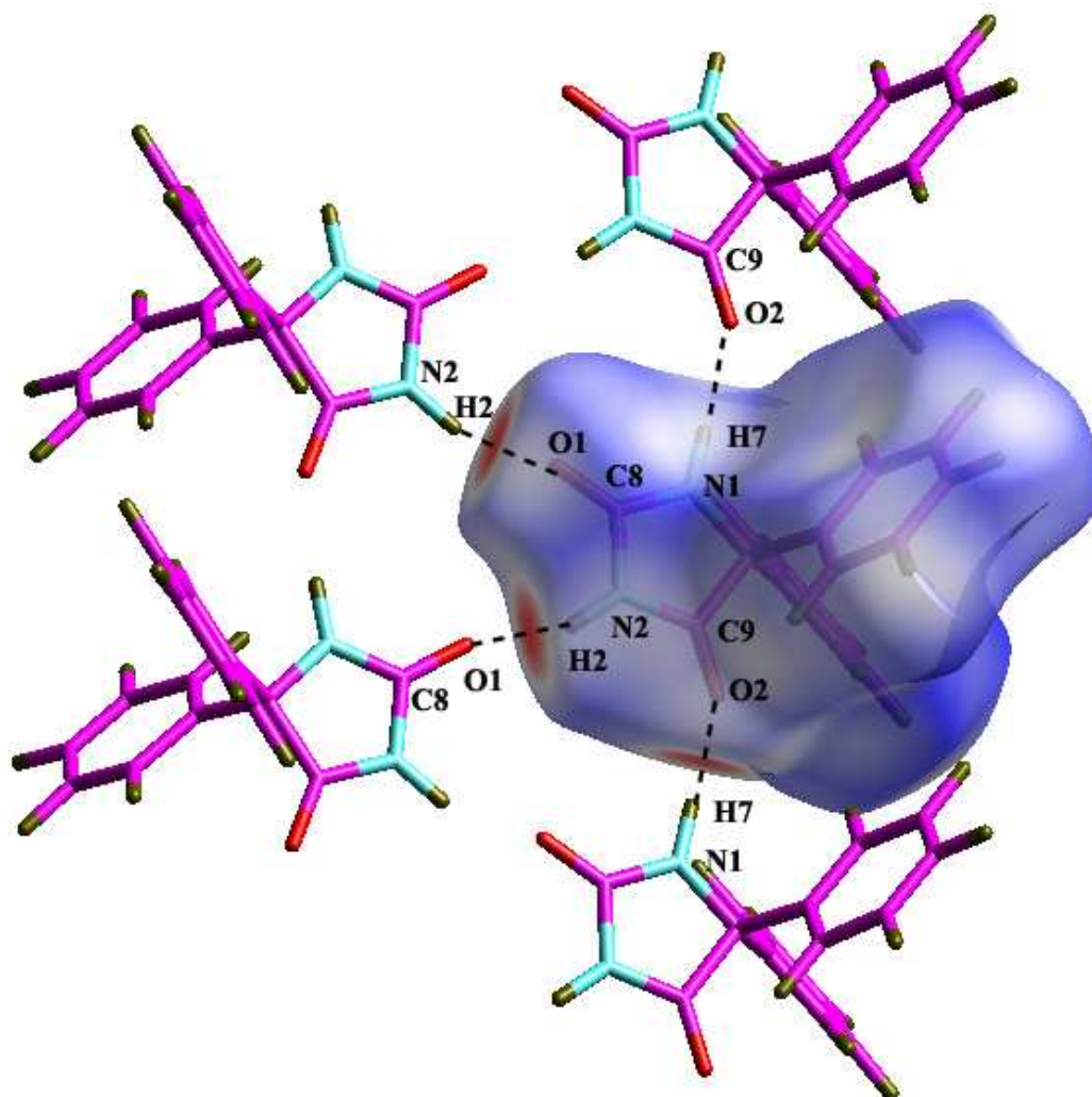
Hirshfeld surface of dilantin molecule.
