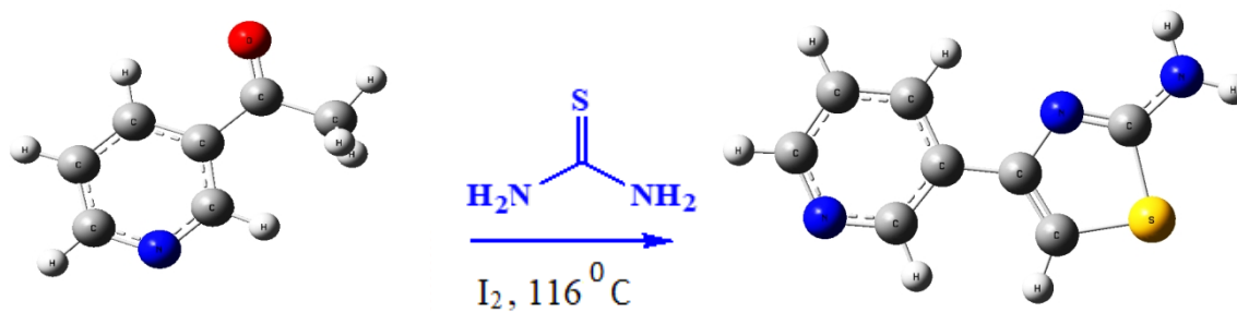
3-acetylpyridine and its 2-aminothiazole product
